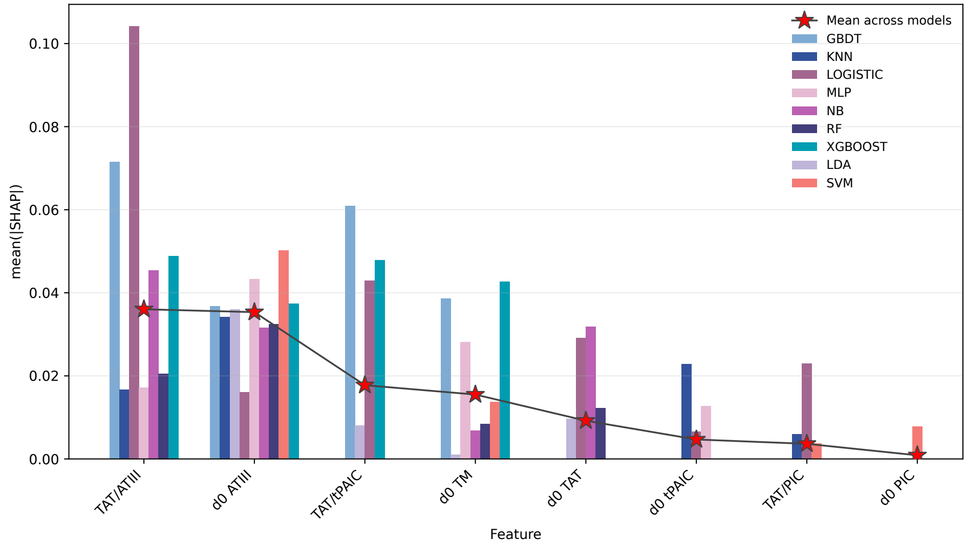
SHAP feature importance for Pre-DIC 1-3
